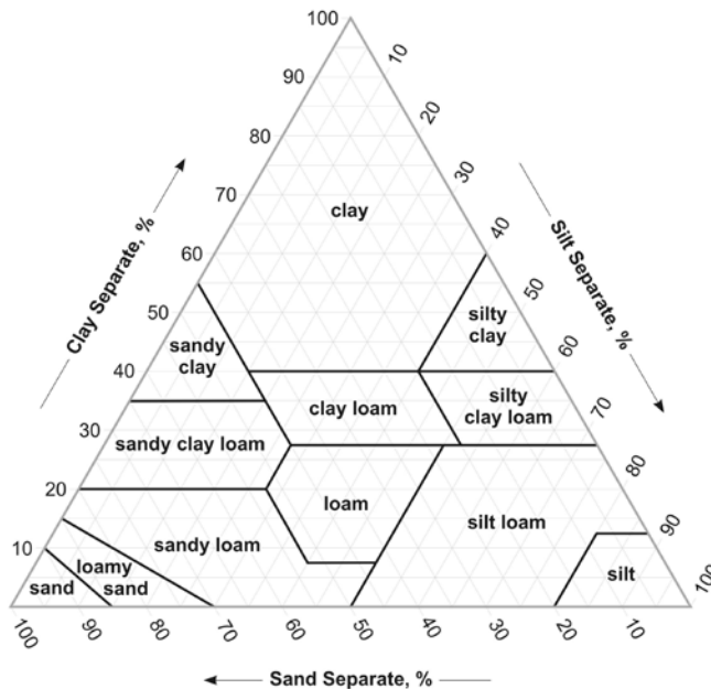
Figure 2.2. Soil textural triangle used for determining soil texture.
