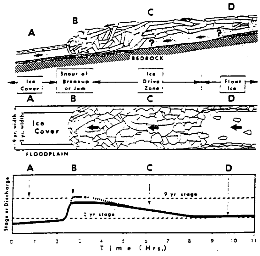
Fig. 2.1 Stages of ice break-up and drive over distance and time (reproduced from Smith, 1980).
