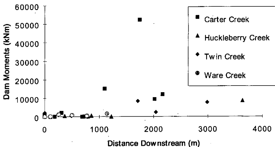
Fig. 5.9 Calculated dam moments as a function of distance downstream from the initiation point.
