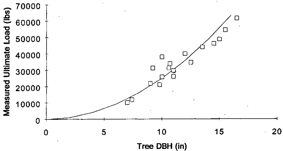
Fig. 5.5 Relationship between ultimate load and tree diameter breast height (DBH).
