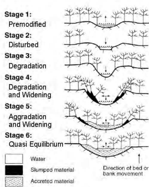
Figure 42. Channel incision and vertical channel change over time (Drawing: modified from Simon and Hupp 1986).
