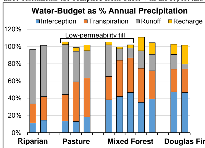
Figure 1. Water-budget components for each cover type. Riparian areas were zones of groundwater emergence and, therefore, had no recharge.
