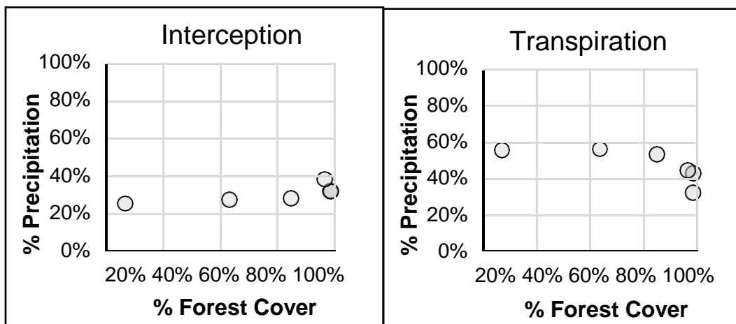
Figure 1. Interception losses, transpiration, and evapotranspiration as a proportion of total precipitation averaged over water years 1997-98 plotted as a function of % forest cover (conifer + deciduous).
